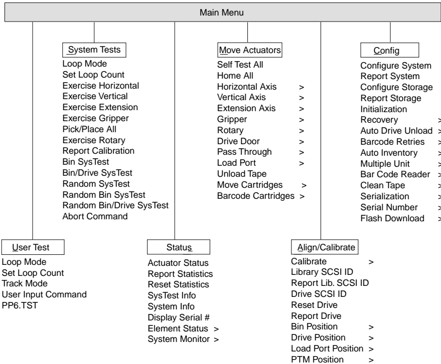
Figure 6-2. Diagnostic software menu options
