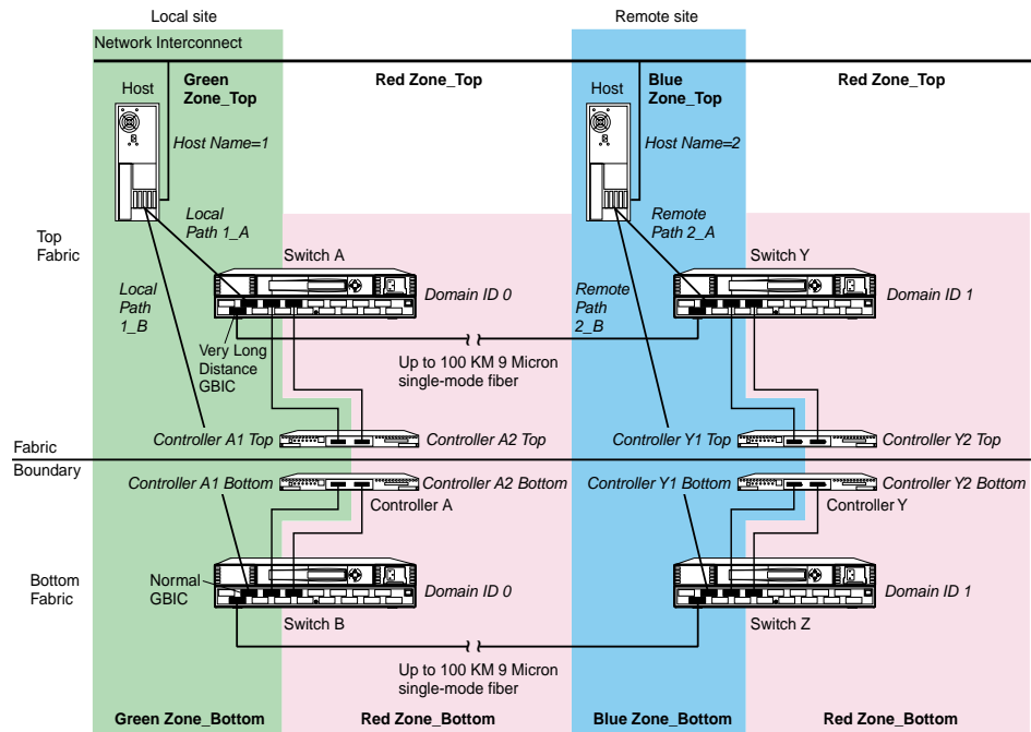
Figure 7-8. Zoning a DRM example
