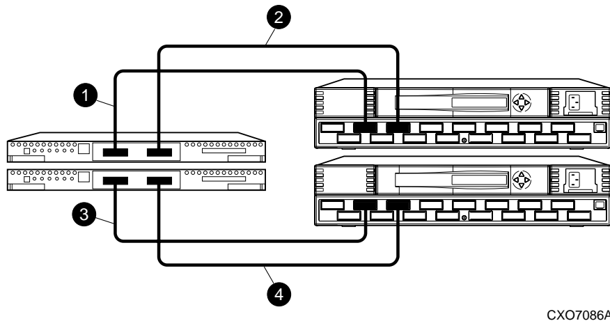
Figure 4-3. Cabling between the controllers and switches
