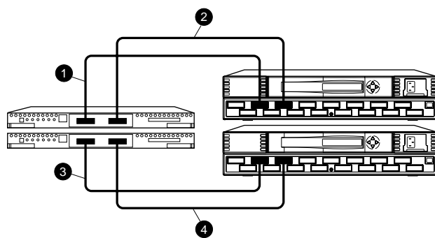
Figure 4-8. Cabling between the controllers and Fibre Channel switches
