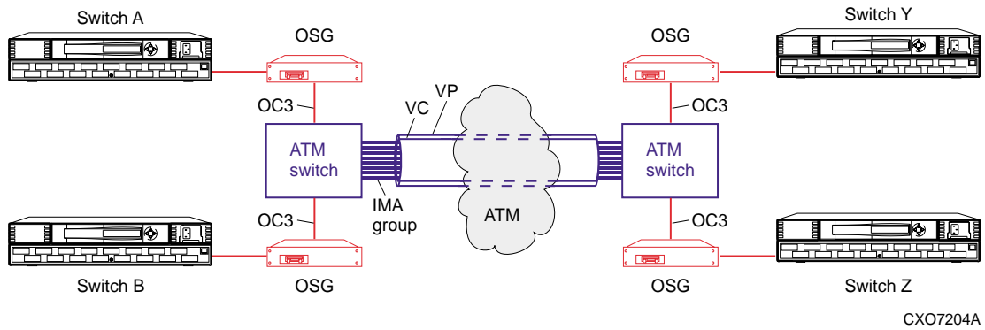
Figure 5 ATM inverse multiplexing configuration
