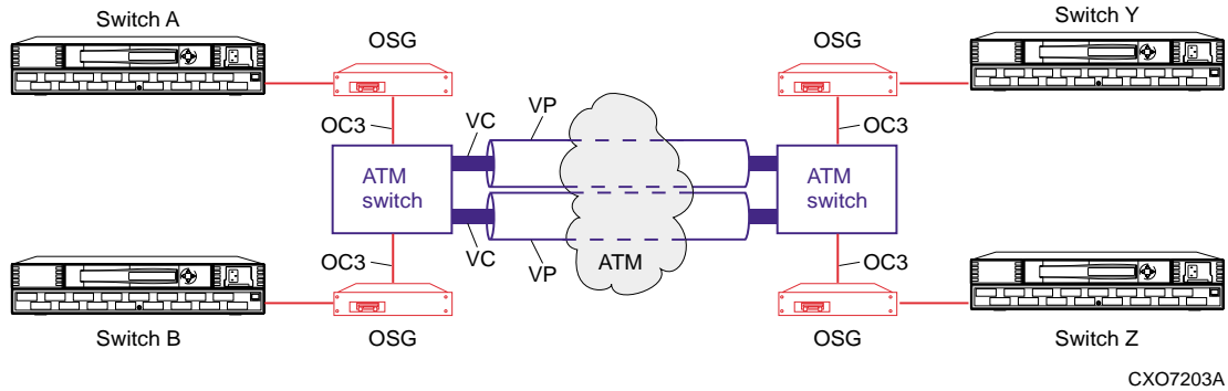
Figure 4 Fractional virtual channel link configuration
