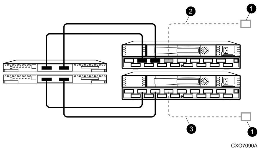
Figure 4-7. Cabling from the initiator site to the target site
