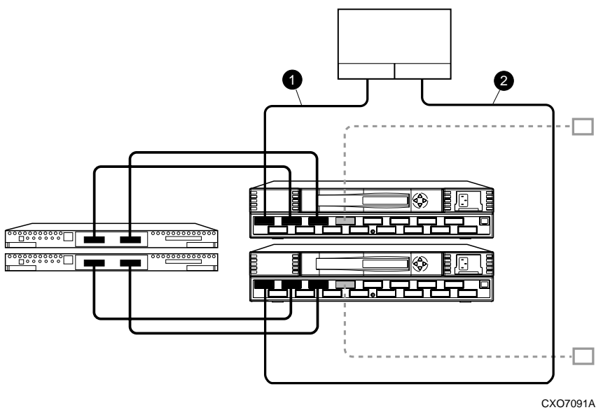
Figure 4-8. Cabling between the hosts and the switches
