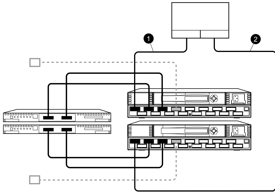
Figure 4-4. Cabling between the hosts and the switches
