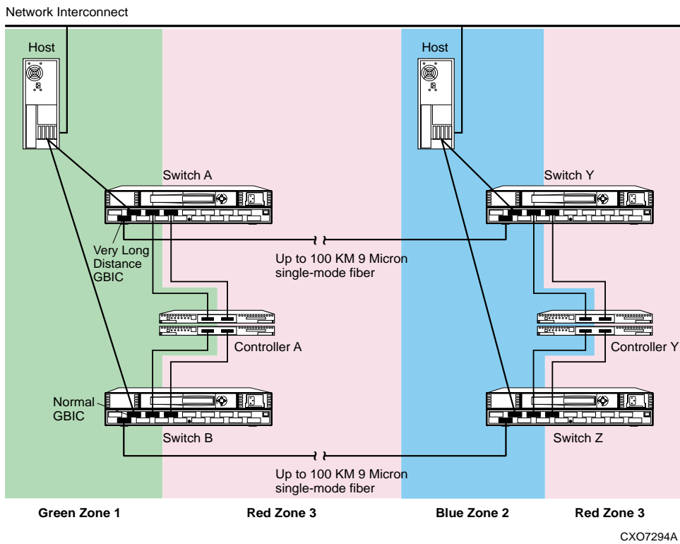
Figure 7-6. Zoning in DRM homogeneous environment
