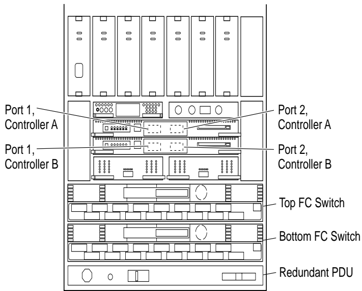
Figure 3-1. Locations and names of components for connecting fiber optic lines
