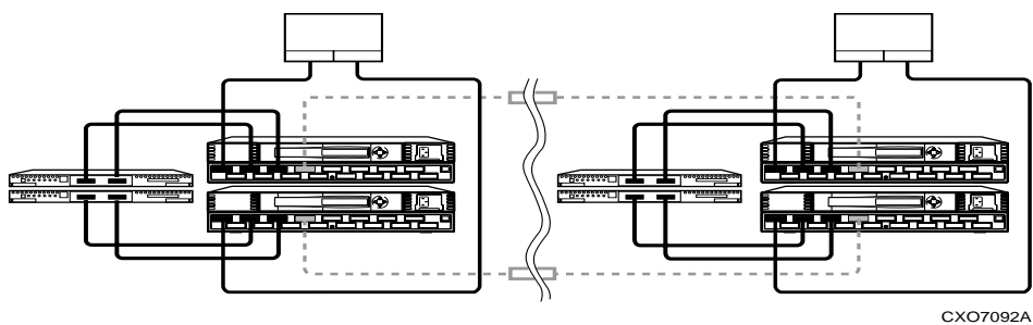
Figure 4-9. Data Replication Manager cabling at initiator and target sites
