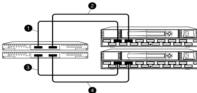
Figure 4-6. Cabling between the controllers and switches
