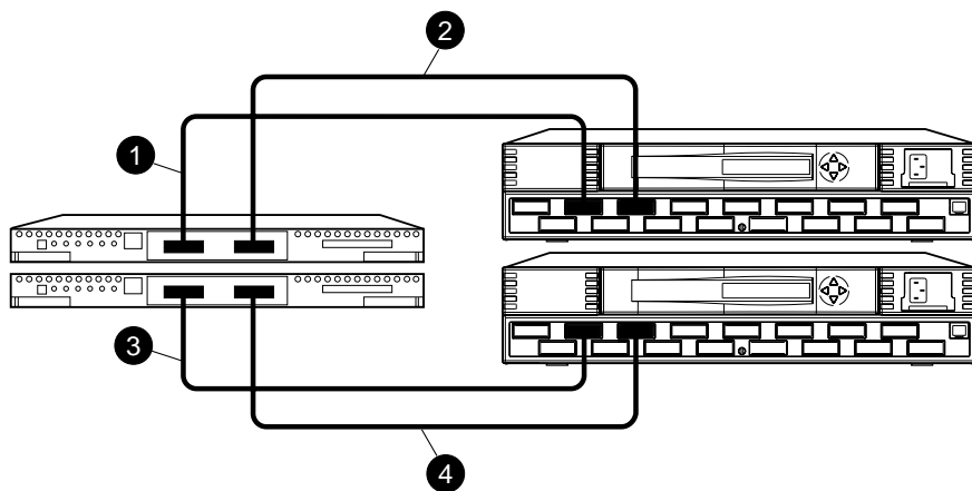
Figure 4-2. Cabling between the controllers and switches
