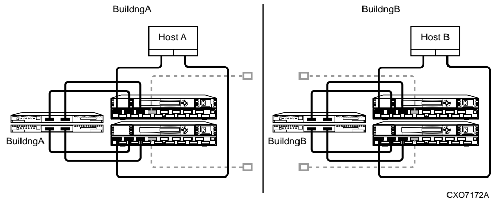
Figure 4-1. Data Replication Manager basic configuration
