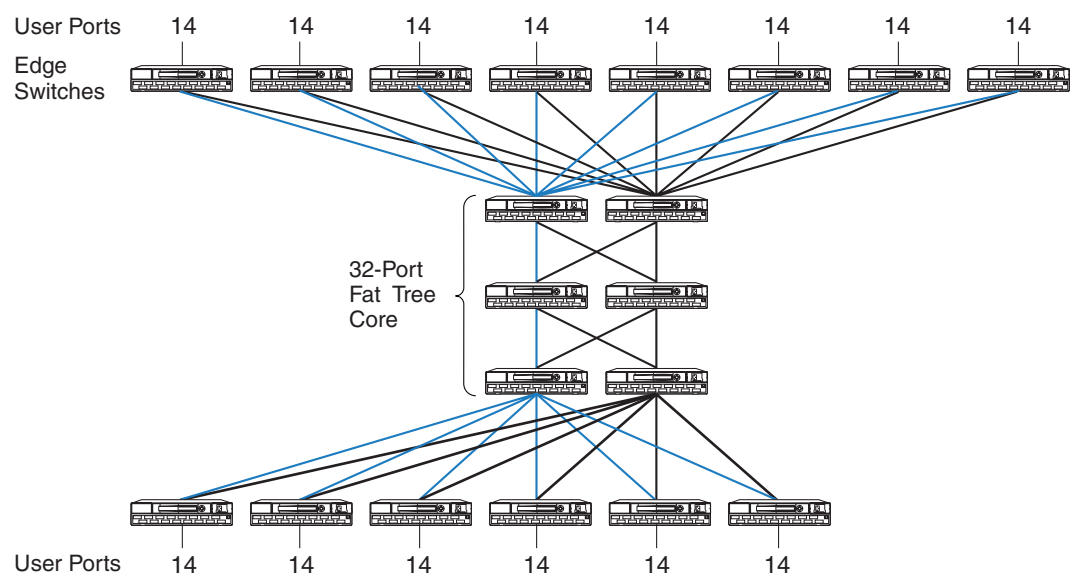
Figure 61: Example of Core Switch Plus Edge Switch Configuration
