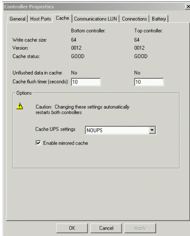
Figure 2-9. Cache controller properties tab
