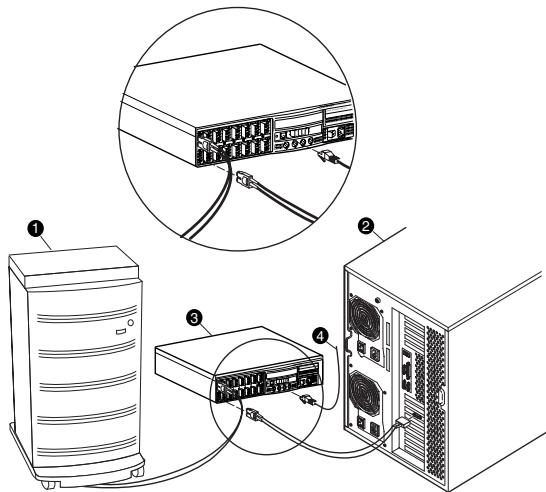
Figure 1-4. Connect the Fibre Channel Adapter to the HSG80 Controller (using a switch and the RA8000)
