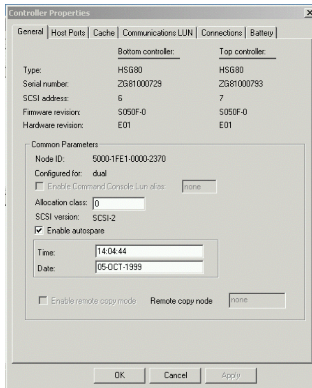
Figure 2-6. General controller properties tab
