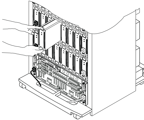
Figure 1-1. Installing SBBs into Storage System Cabinet
