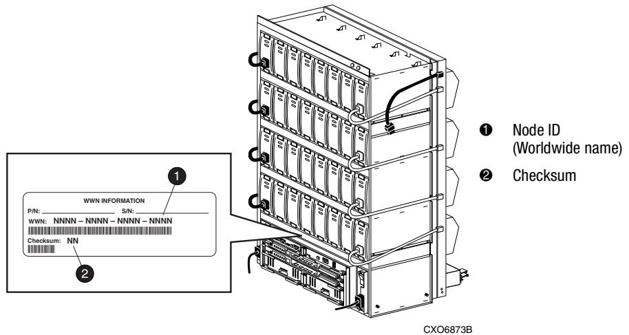
Figure 1-9. Placement of the worldwide name label on the Model 2200 enclosure
