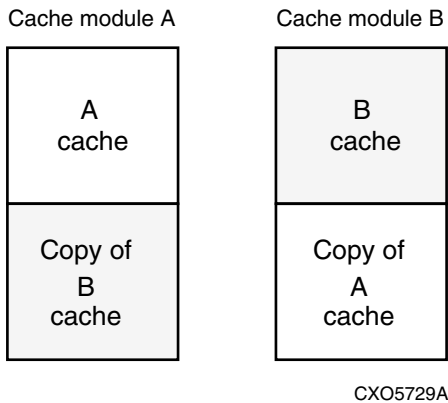
Figure 1-6. Mirrored caching
