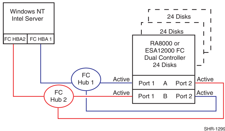
Figure 1 HA Configuration 1
