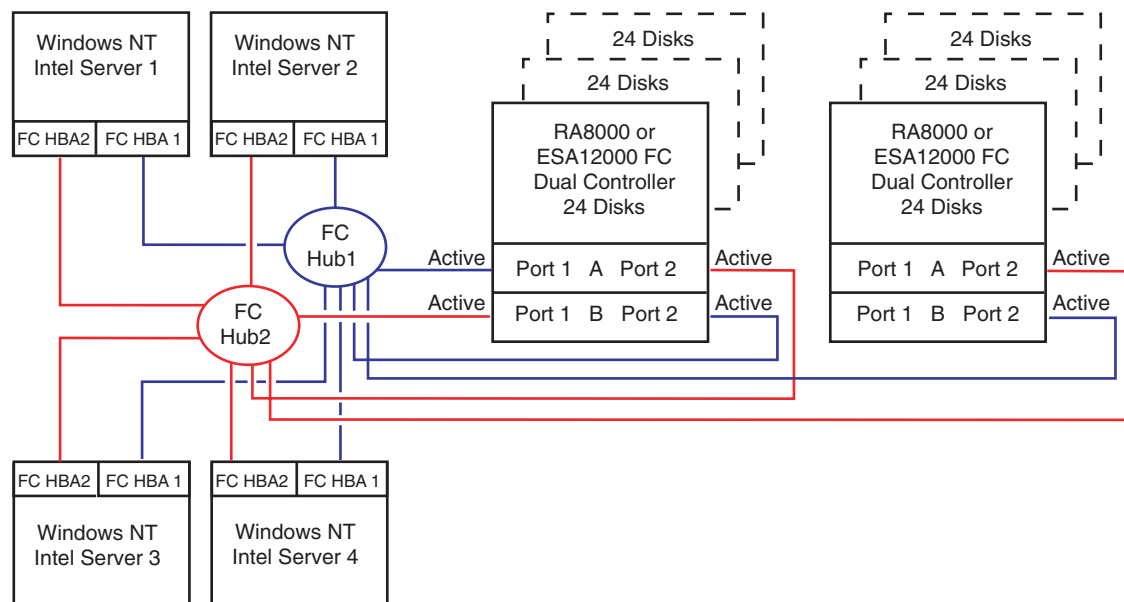
Figure 9 HA Configuration 8
