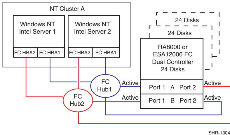
Figure 5 HA Configuration 4
