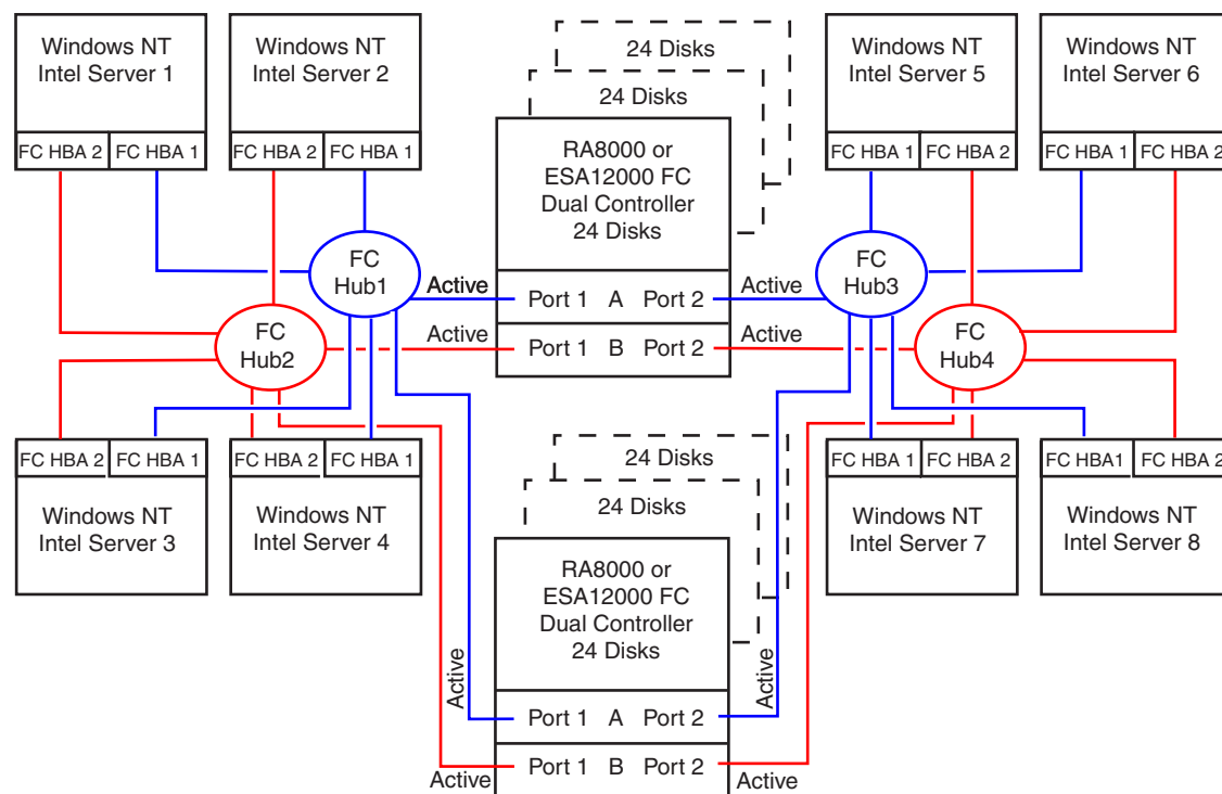
Figure 10 HA Configuration 9
