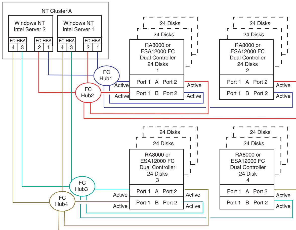
Figure 6 HA Configuration 5
