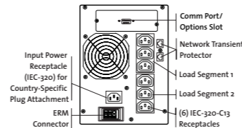
UPS T1000 XR, INTL/ UPS T1500 XR, INTL
