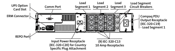
UPS R3000 XR, IEC-309
