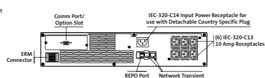
UPS R1500 XR, INTL
