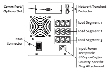
UPS T2200 XR, INTL
