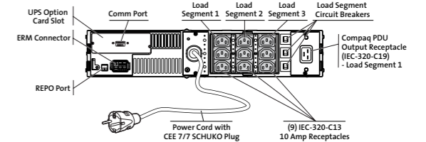
UPS R3000 XR, South Africa Plug
