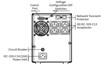
UPS T700, INTL
