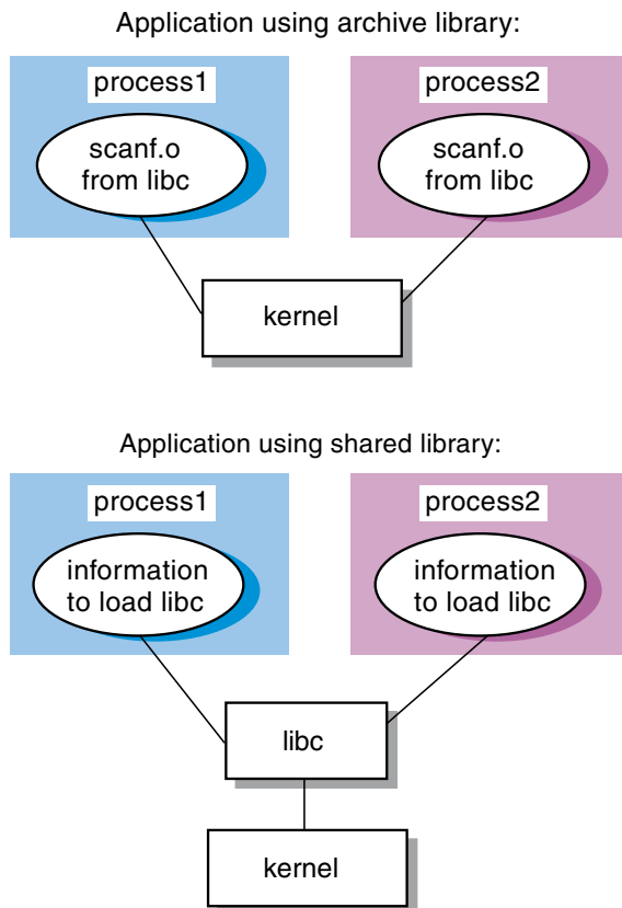
Figure 3–1: Use of Archive and Shared Libraries
