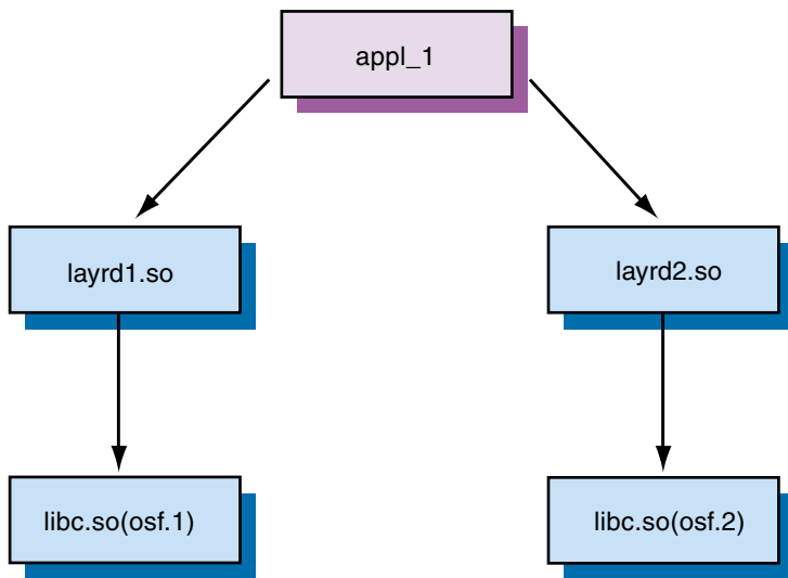
Figure 3–3: Invalid Multiple Version Dependencies Among Shared Objects: Example 1
